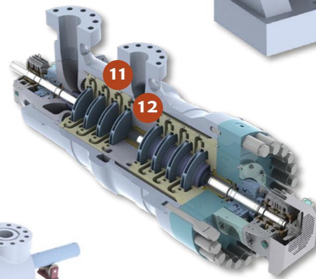
CUP - BB5 (back-to-back impeller arrangement)
