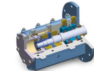
Optional sleeve/tilting pad bearing assembly
