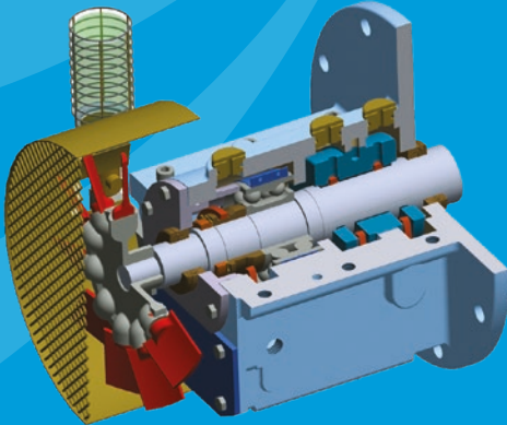
Optional sleeve/ ball bearing assembly
