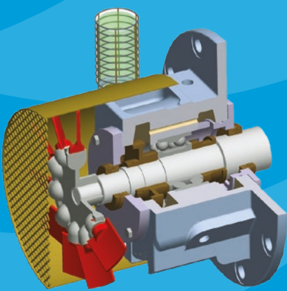
Standard ball /ball bearing assembly
